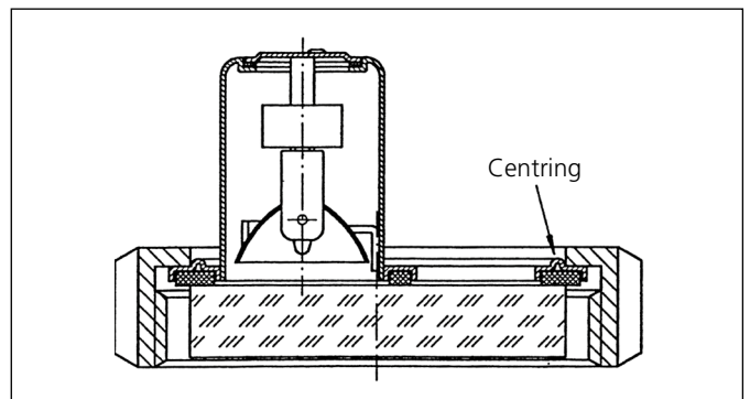
Lumistar luminaire ME, stainless steel
