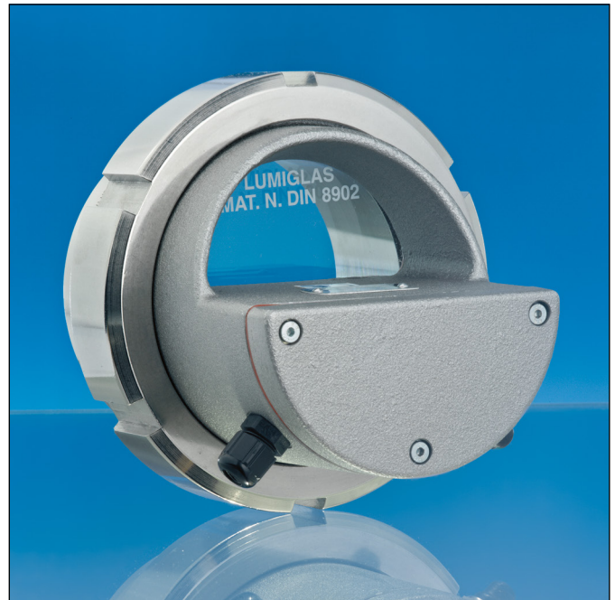
Lumistar luminaire SLM built in a screwed sight glass fitting
